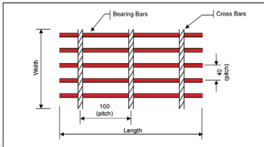
Figure 14 – Gratings: Dimensions
